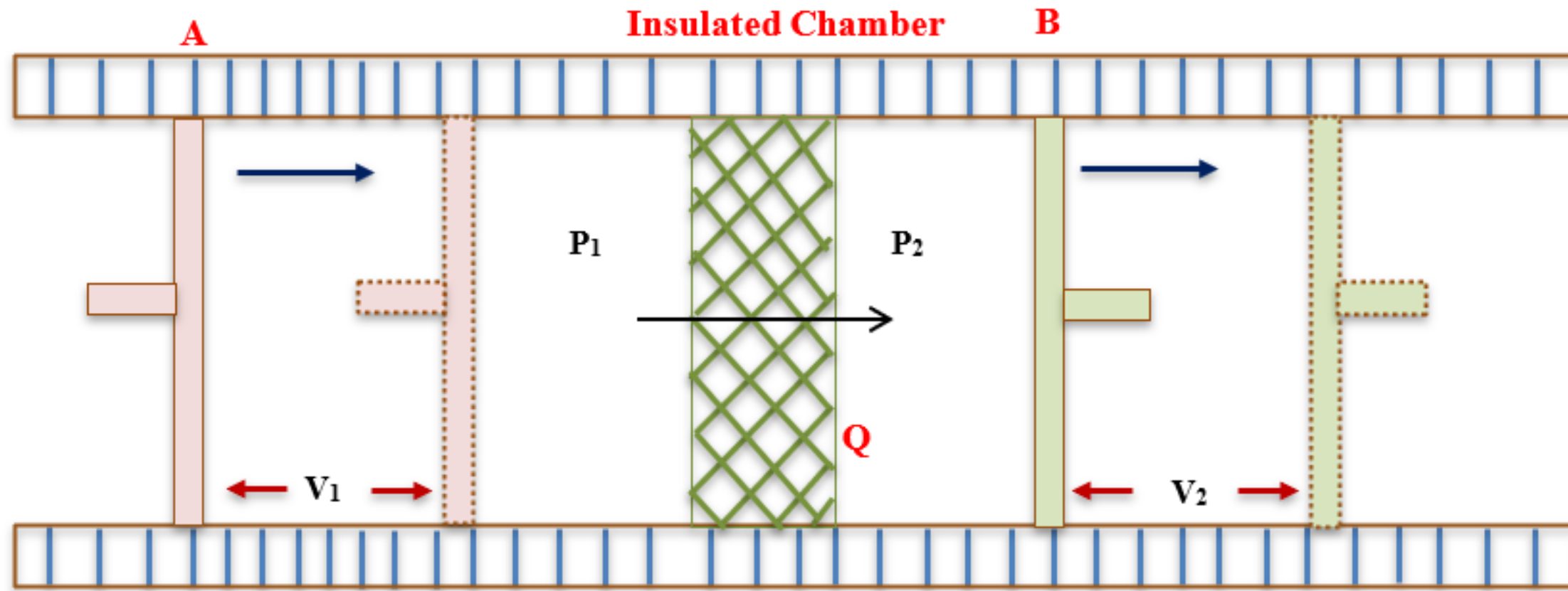
Joule-Thomson experiment (expansion of a real gas through a porous plug)
