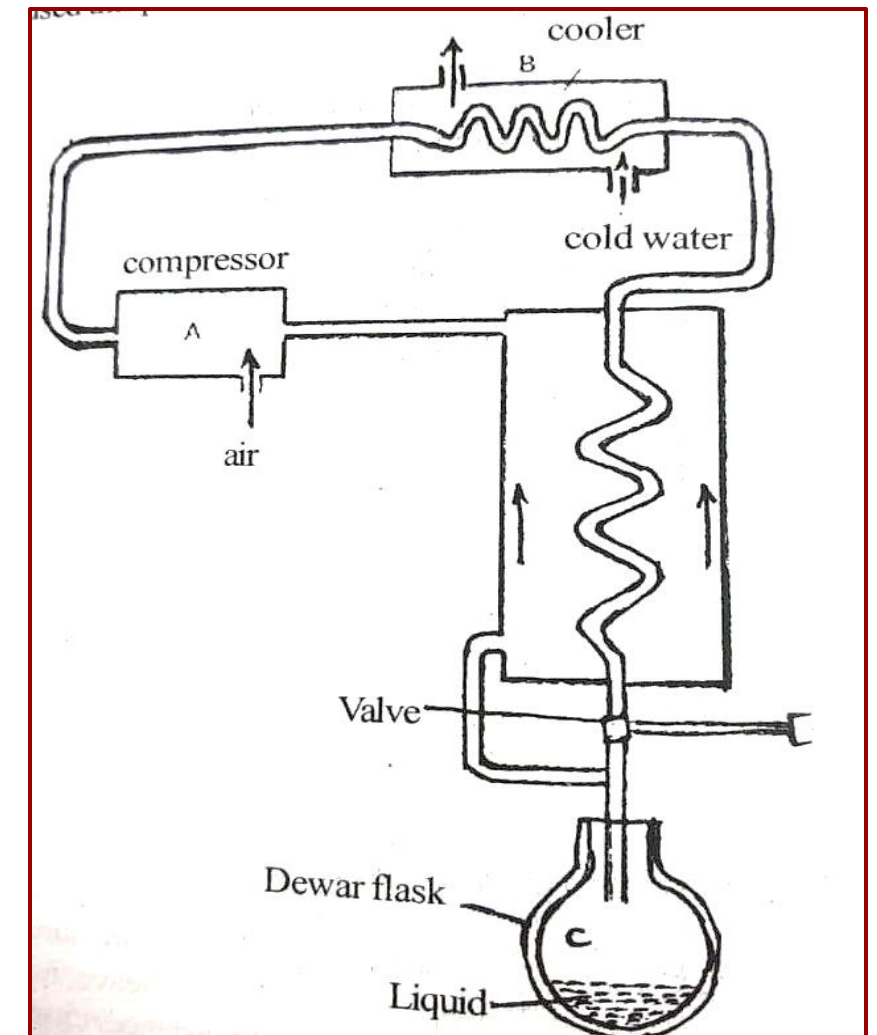
Linde liquefaction Unit
